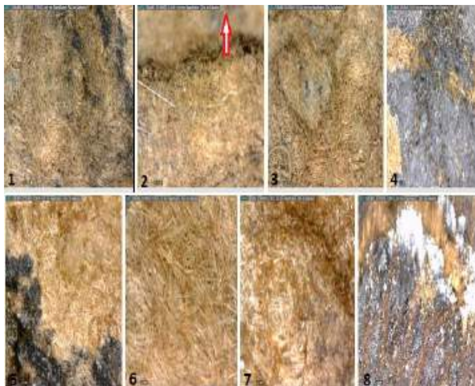
[FIGURE 4]: Examining the archaeological leather document sample with magnification 230x, 1280x960 no calibration as the arrow indicates the image; 1-8: using Digital light microscope (Dino light) for examining which explain deformation of the surface morphology in different places.
