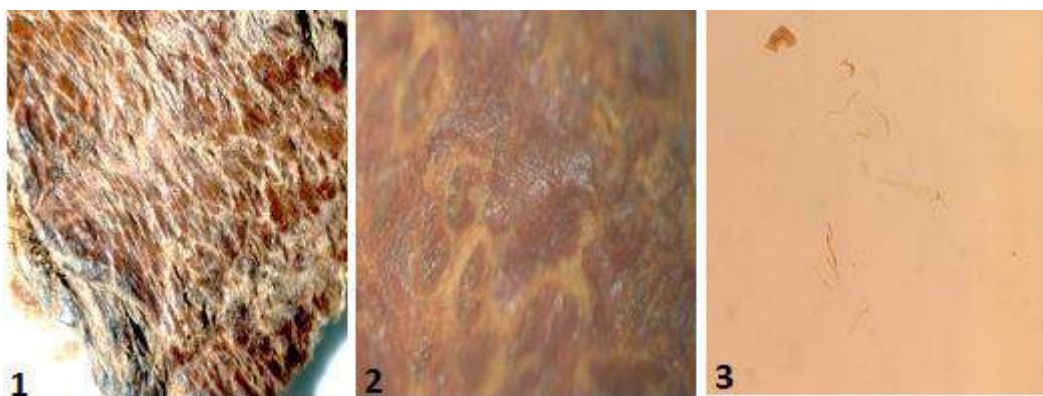
[FIGURE 6]: Examining the archaeological leather document sample; 1-3: using polarizing microscope (P.M.) for examining the surface morphology with magnification 1-50x; 2-100x; 3-25x.
